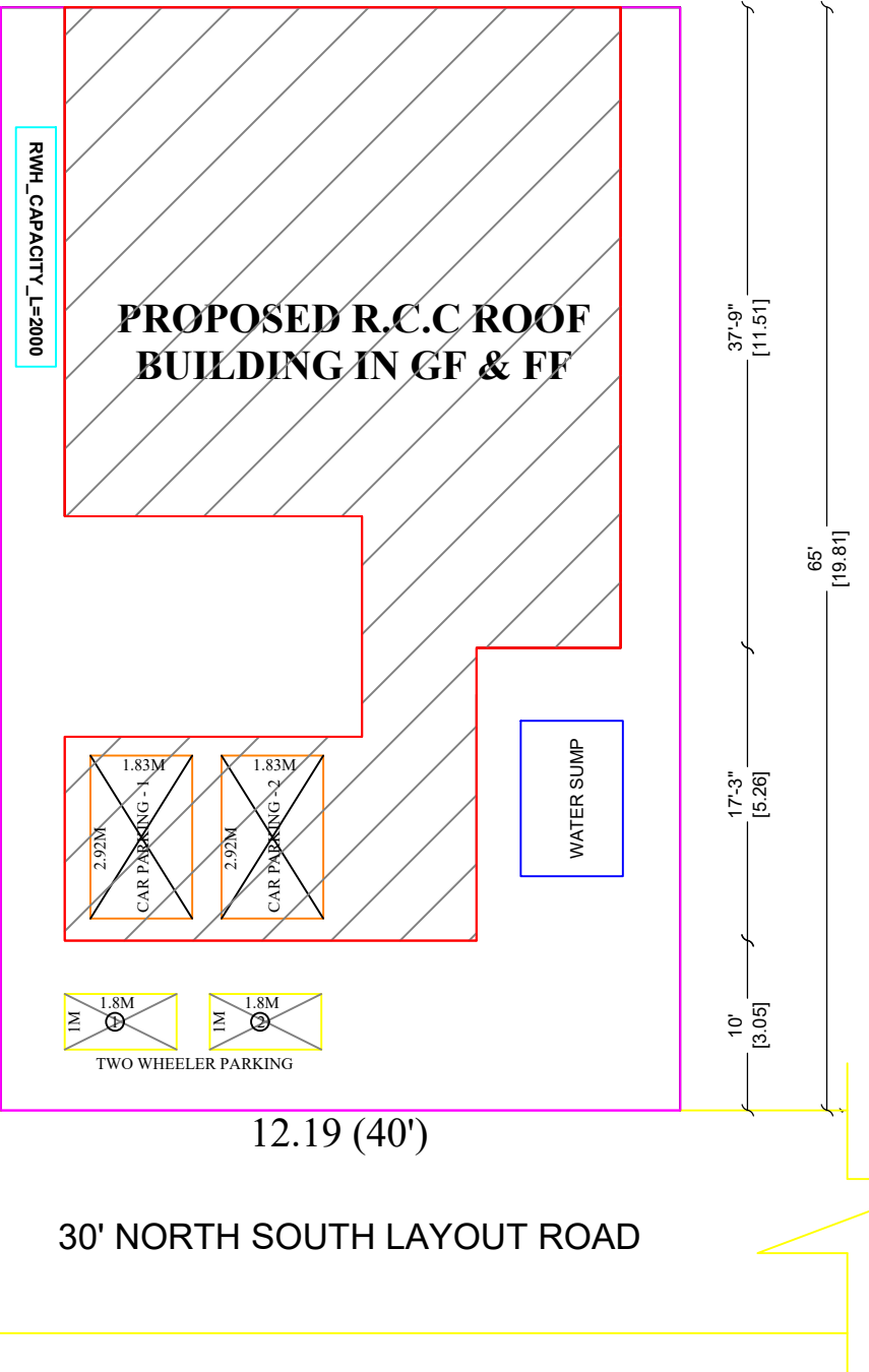
SITE PLAN
