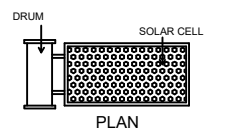
SOLAR WATER HEATER DETAIL (NTS)
