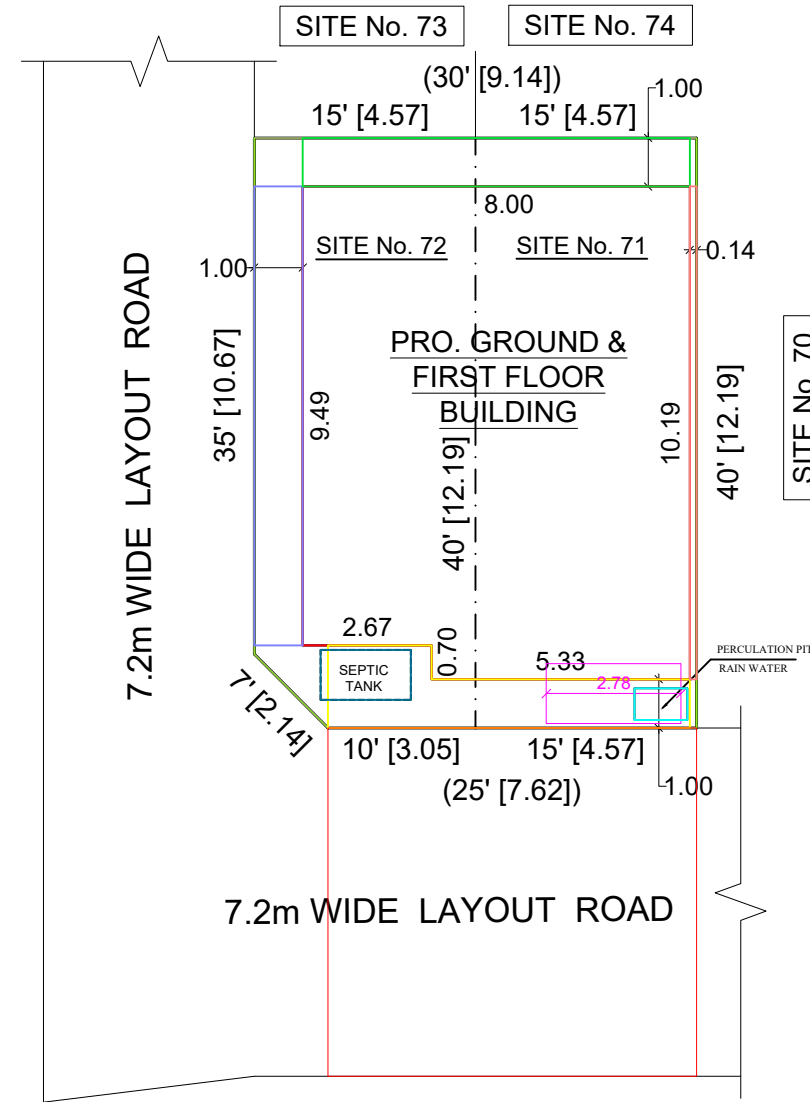
SITE PLAN
