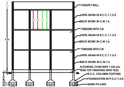
SECTION-AB
