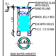
RAIN WATER HARVEST
