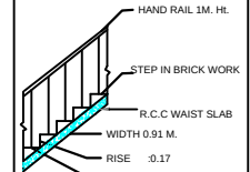
STAIR DETAIL
