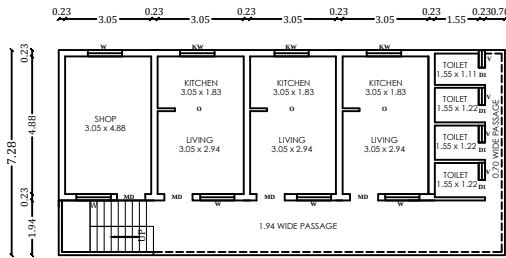
PRO.ADDITIONAL & ALTERATION OF G.FLOOR
