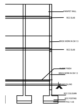
SECTION ON A B
