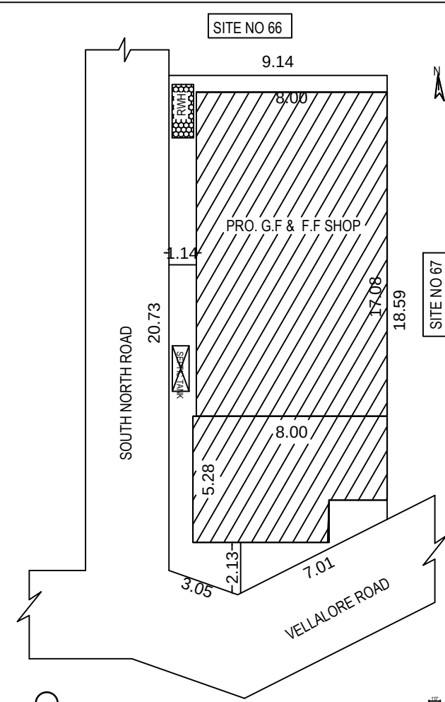
SITE PLAN
