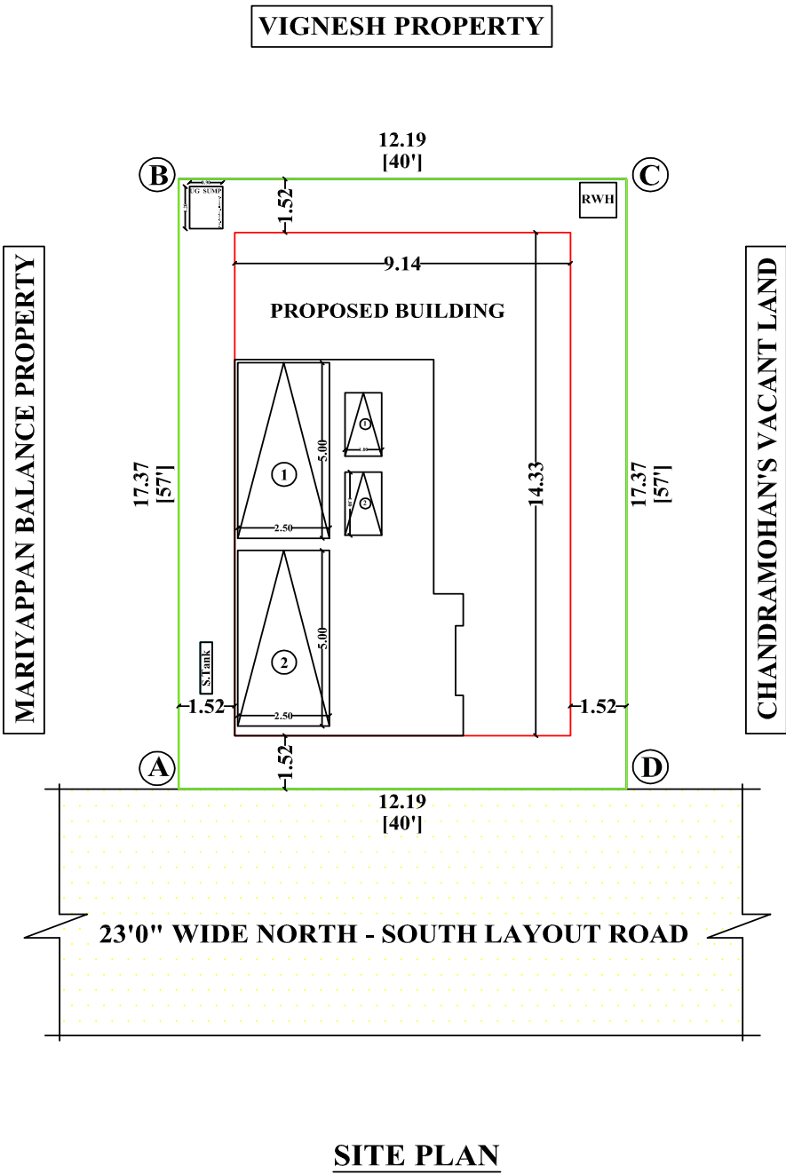
SITE PLAN
