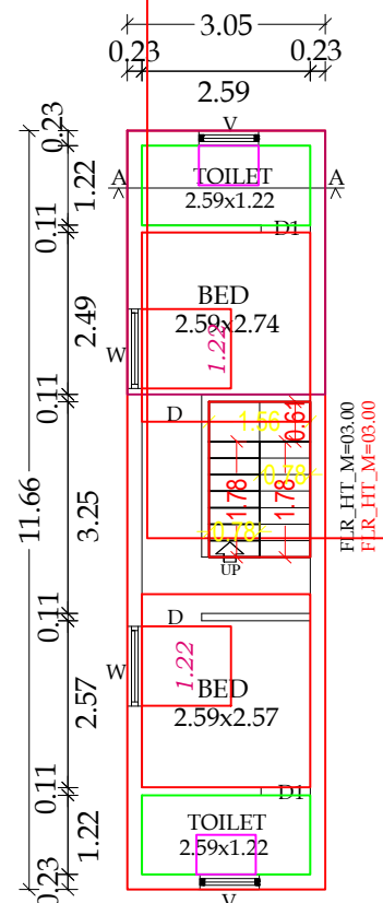
SECOND FLOOR
