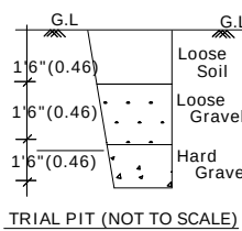
TRIAL PIT (NOT TO SCALE)
