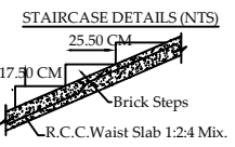
STAIRCASE DETAILS (NTS)
