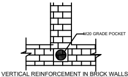
VERTICAL REINFORCEMENT IN BRICK WALLS
