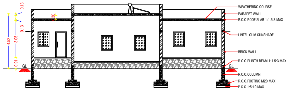
SECTION - AA @ SOUTH SIDE VIEW
