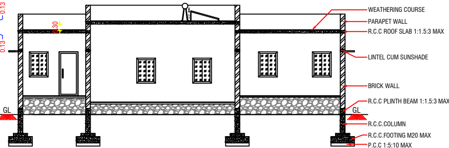
SECTION - AA @ SOUTH SIDE VIEW
