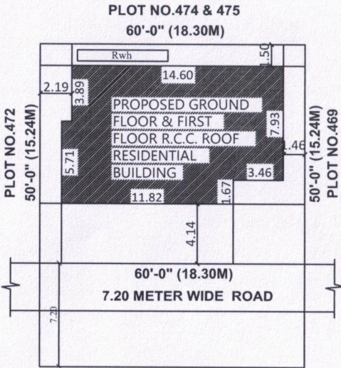
SITE PLAN
