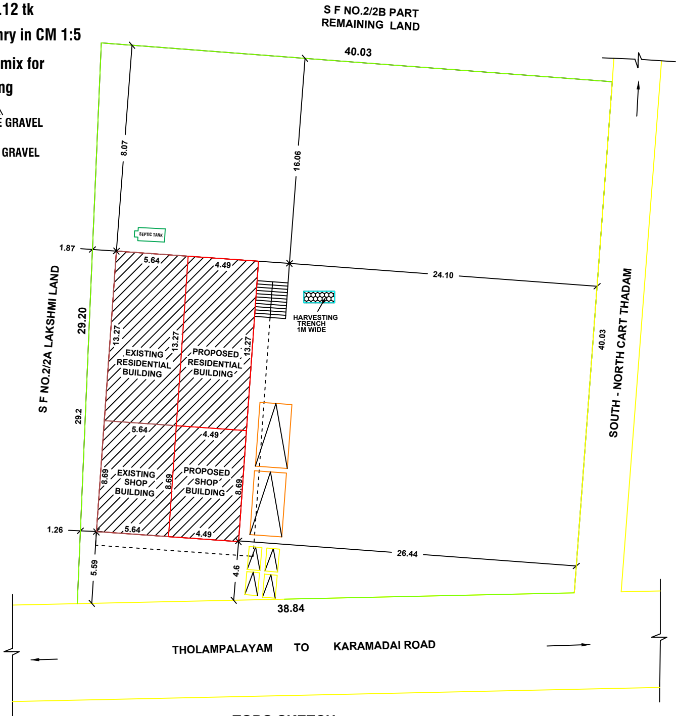
TOPO SKETCH
