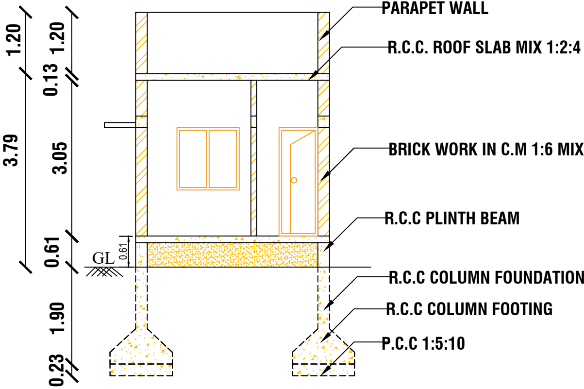
CROSS SECTION AT A-A
