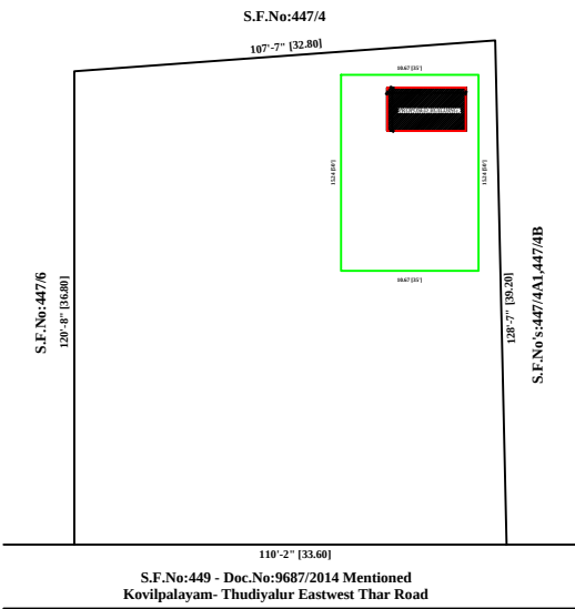
SITE PLAN
