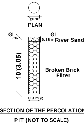
SECTION OF THE PERCOLATION PIT (NOT TO SCALE)
