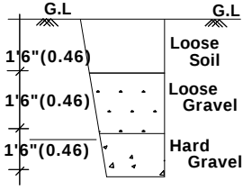
TRIAL PIT (NOT TO SCALE)
