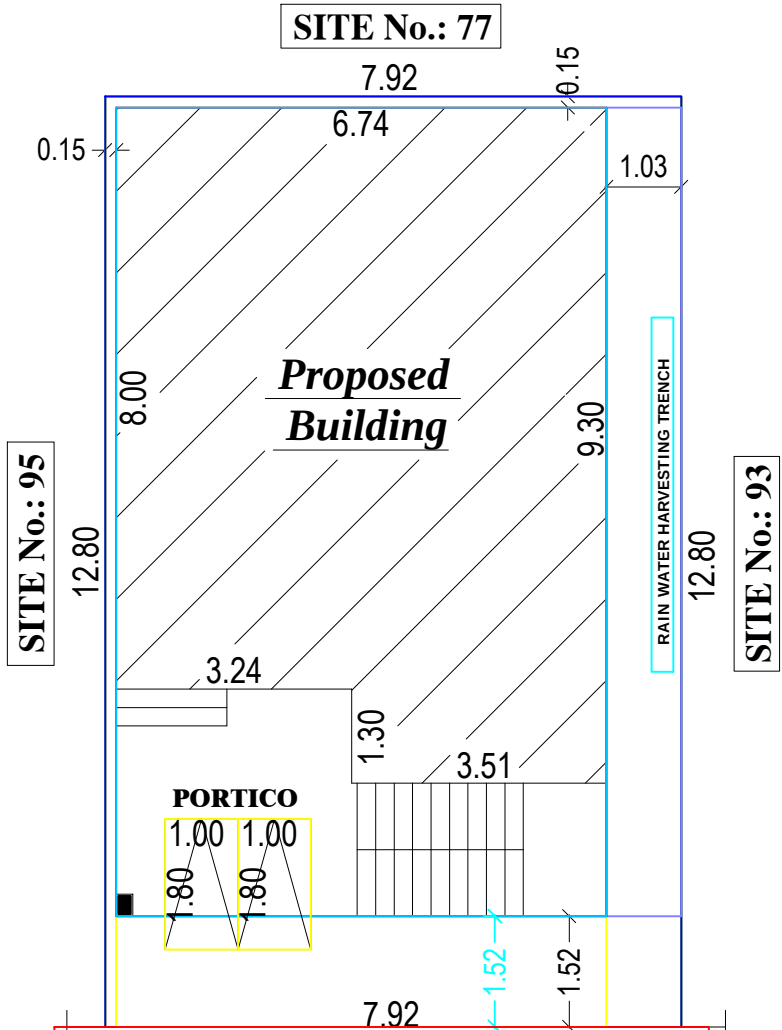
SITE PLAN
