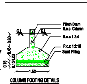
COLUMN FOOTING DETAILS
