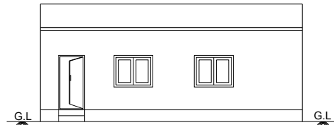
FRONT ELEVATION
