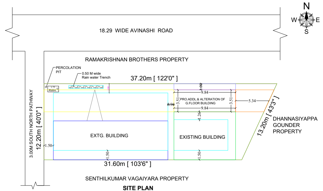
SITE PLAN
