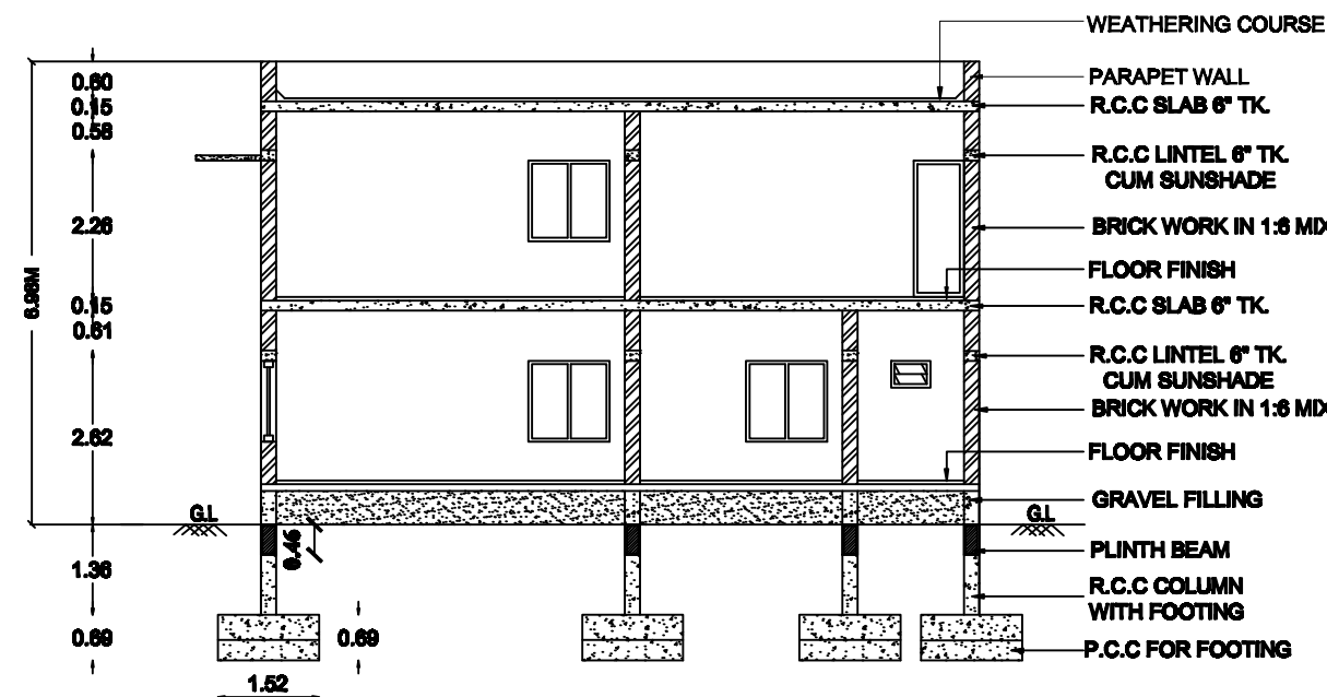
CROSS SECTION AT A-A
