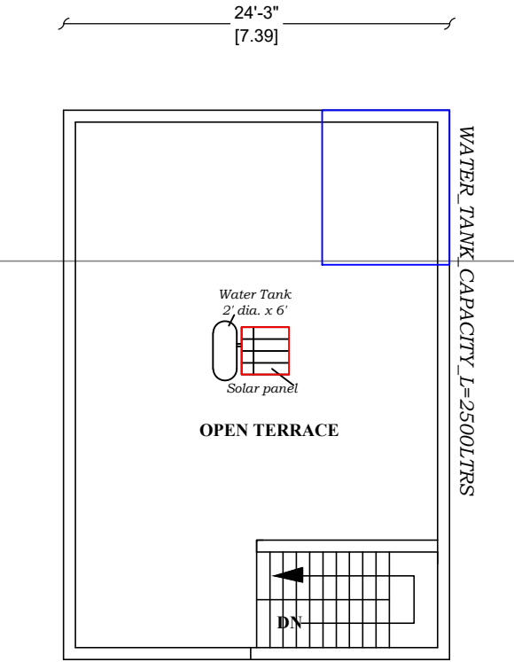
PRO. TERRACE FLOOR PLAN
