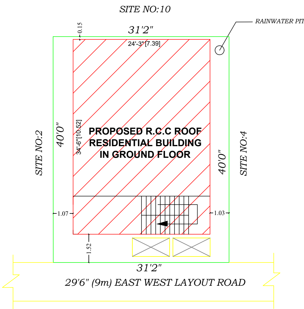
SITE PLAN
