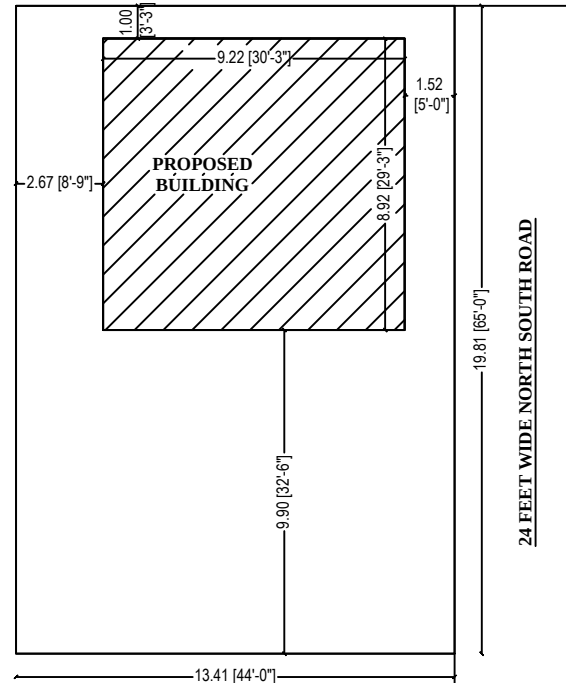
SITE PLAN
