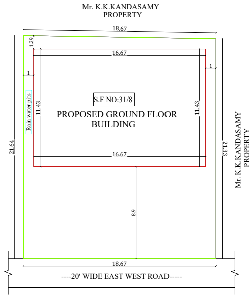
SITE PLAN
