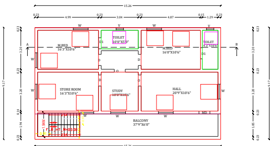
Proposed Third Floor Plan
