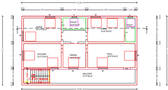
Proposed Second Floor Plan
