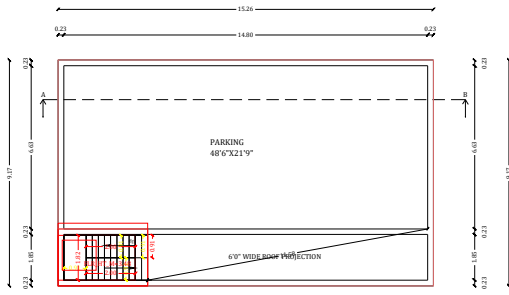
Proposed Stilt Floor Plan
