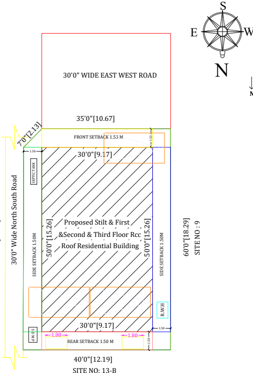
SITE PLAN
