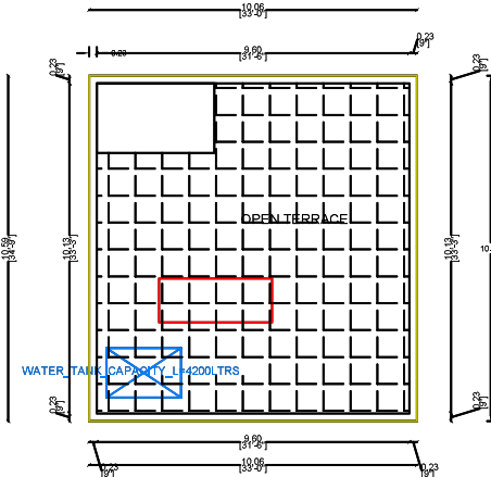
PRO. SECOND FLOOR PLAN.
