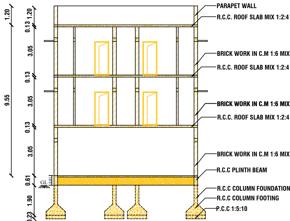
CROSS SECTION AT A-A
