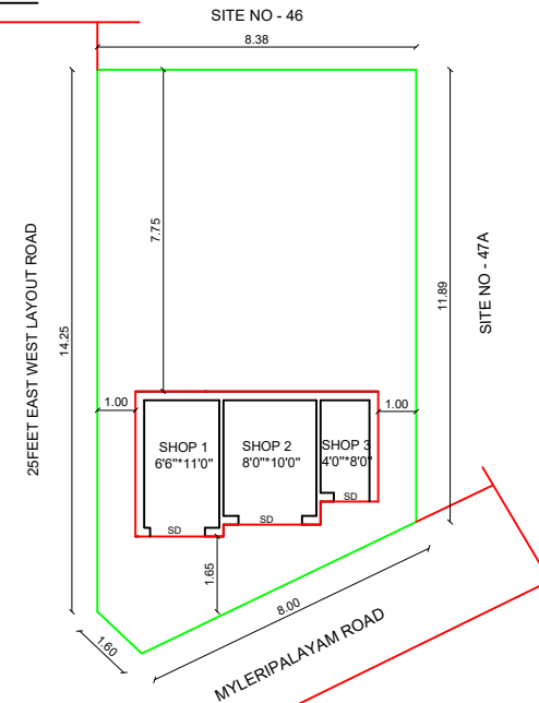
SITE PLAN
