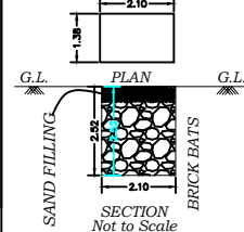
DETAILED PLAN OF RAINWATER PERCOLATION PEBBLE BED RW_CAPACITY_L = 2000LTRS
