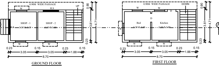
DETAIL PLAN
