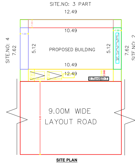
SITE PLAN
