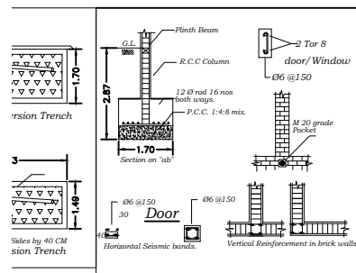
Sectional Elevation of Door and Window Typical Details of Providing Vertical Steel Bars
