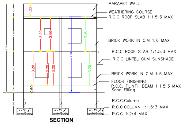
SECTION
