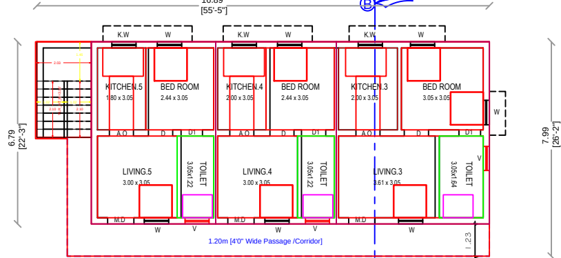
PROP. FIRST FLOOR PLAN
