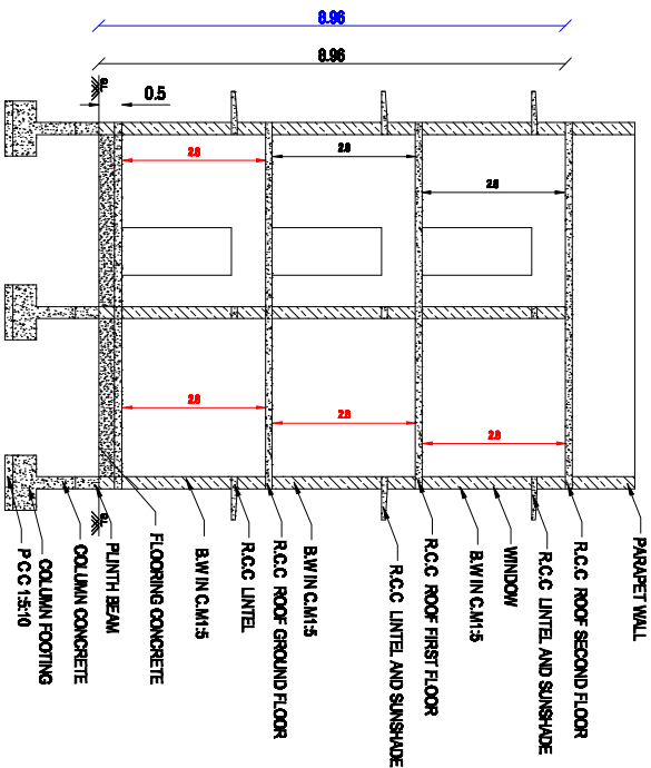
SECTION-AB
