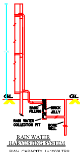
RAIN WATER HARVESTING SYSTEM RWHP_CAPACITY_L=1000LTRS
