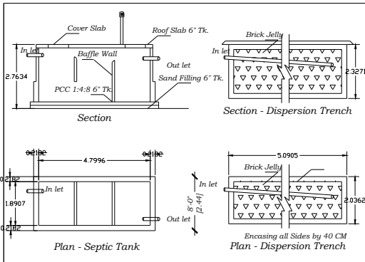
Section - Septic Tank
