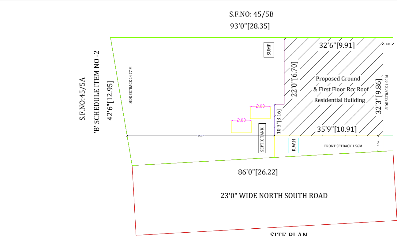
SITE PLAN
