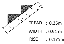
STAIRCASE DETAIL :
