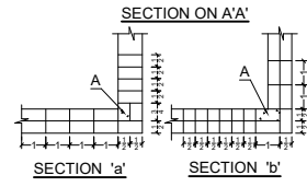
SECTION ON 'A-A' TYPICAL DETAILS OF PROVIDING VERTICAL STEEL BARS IN BRICK MASONRY A : VERTICAL REINFORCEMENT BARS WITH M20 GRADE CONCRETE a & b : ALTERNATE COURSES IN 1 BRICK WALL 1 : ONE BRICK LENGTH 1/2 : HALF BRICK LENGTH 3/4 : THREE QUARTERS BRICK LENGTH
