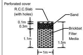
RAIN WATER HARVESTING RECHARGE TRENCH SECTION
