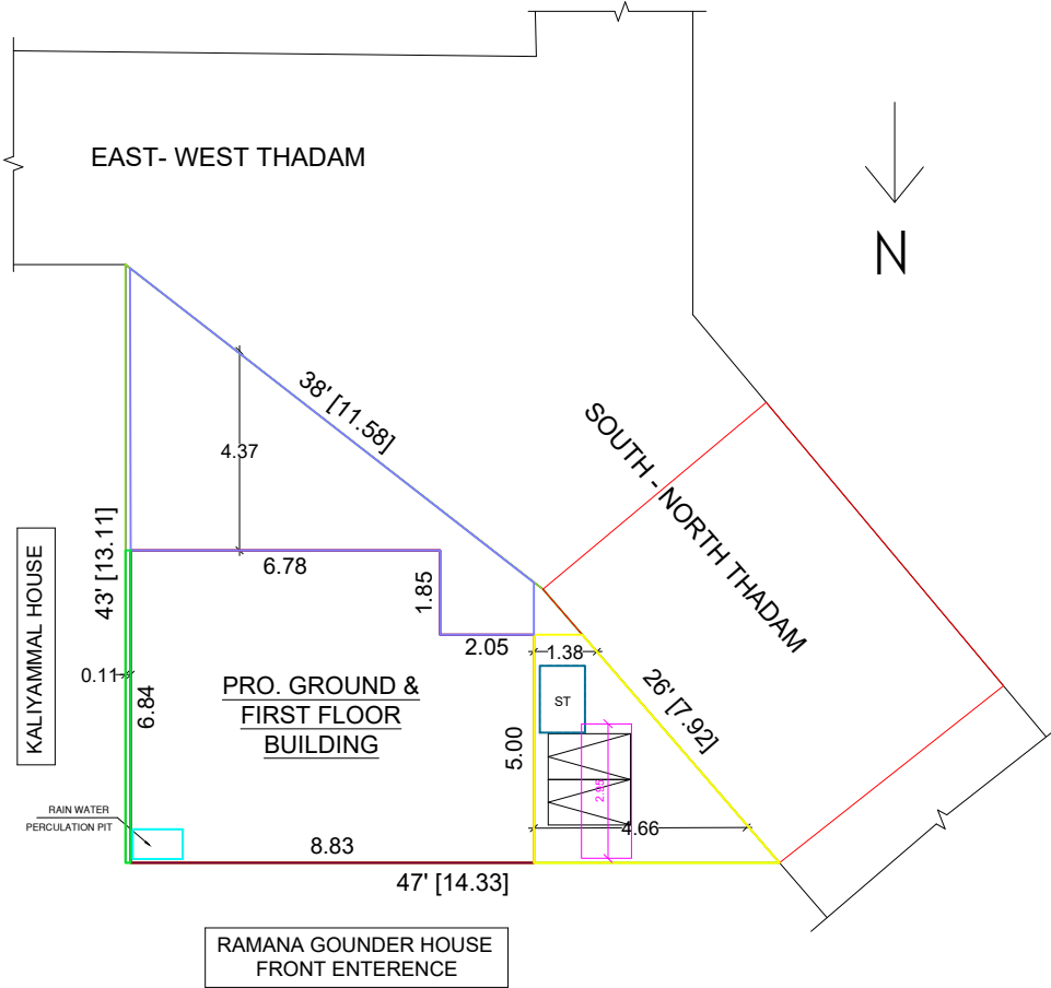
SITE PLAN
