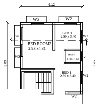
LOOR PLAN
