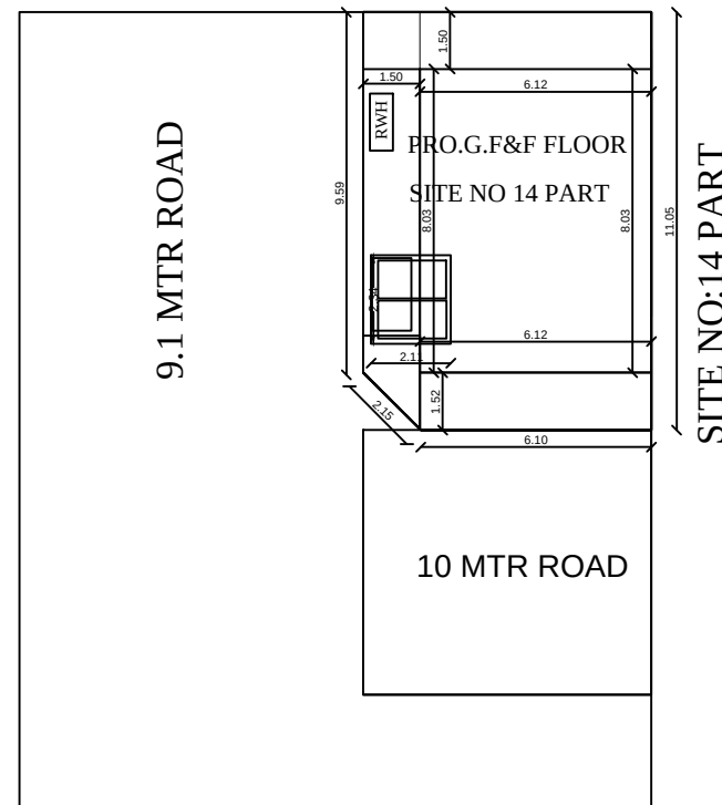
SITE PLAN
