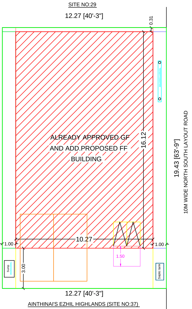
SITE PLAN
