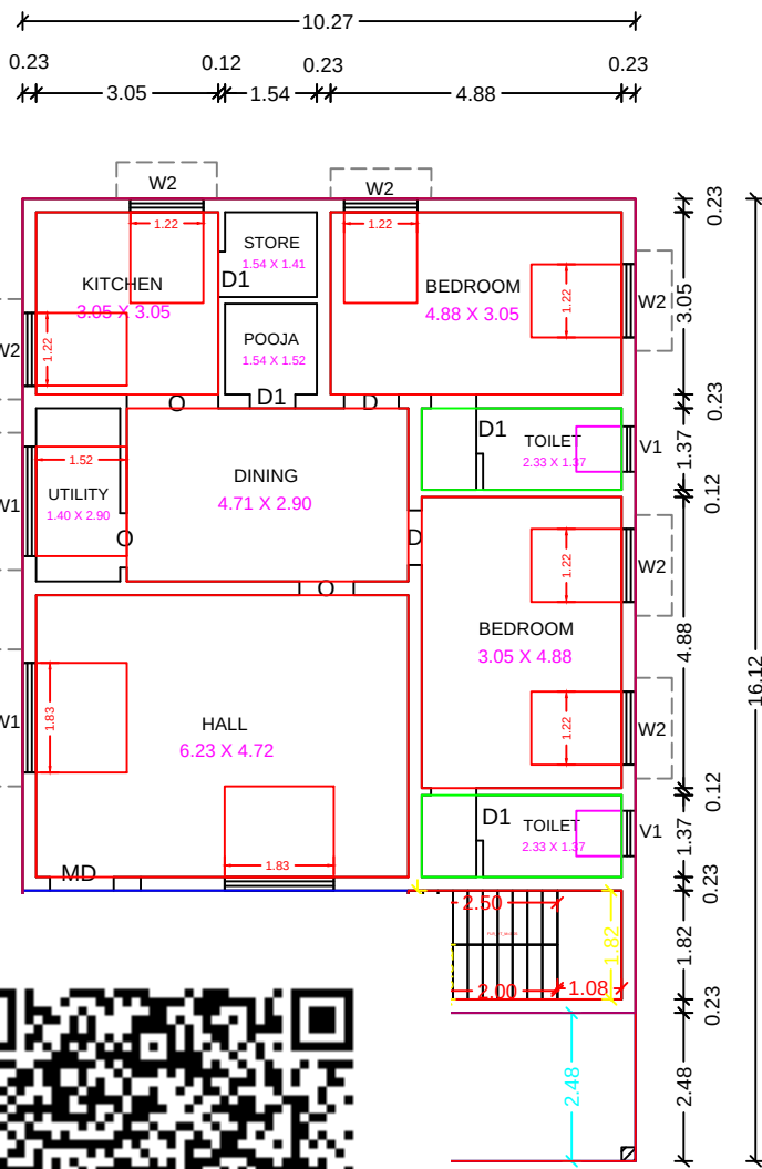
FLOOR PLAN
