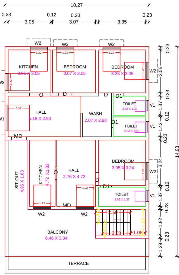
ADD. PROPOSED FIRST FLOOR PLAN
