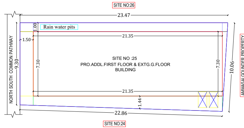
SITE PLAN
