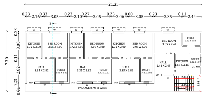
ALTERATION OF EXISTING GROUND FLOOR PLAN
