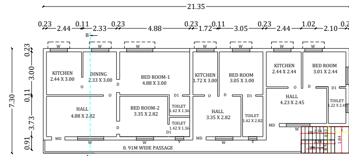
PRO. ADDL FIRST FLOOR PLAN
