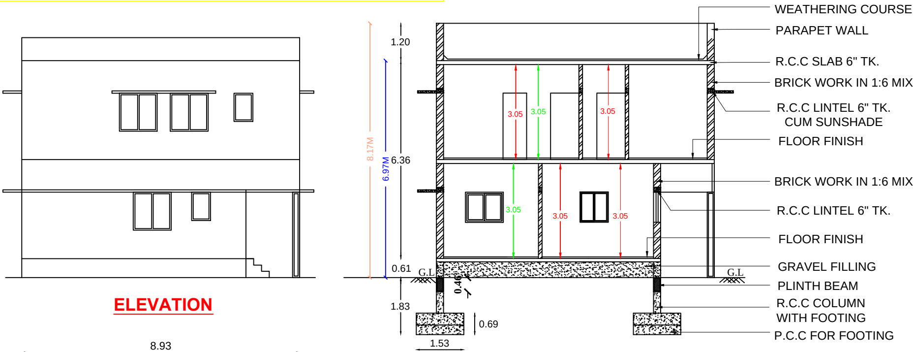
CROSS SECTION AT A-A
