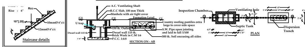
SEPTIC TANK WITH DISPERSION TRENCH (250 Gls.)
