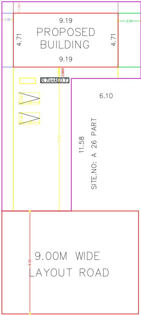
SITE PLAN
