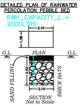
SECTION Not to Scale
