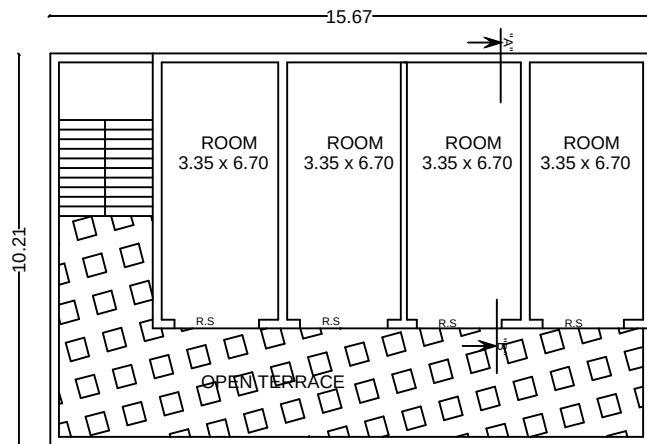
EXG. GROUND FLOOR PLAN
