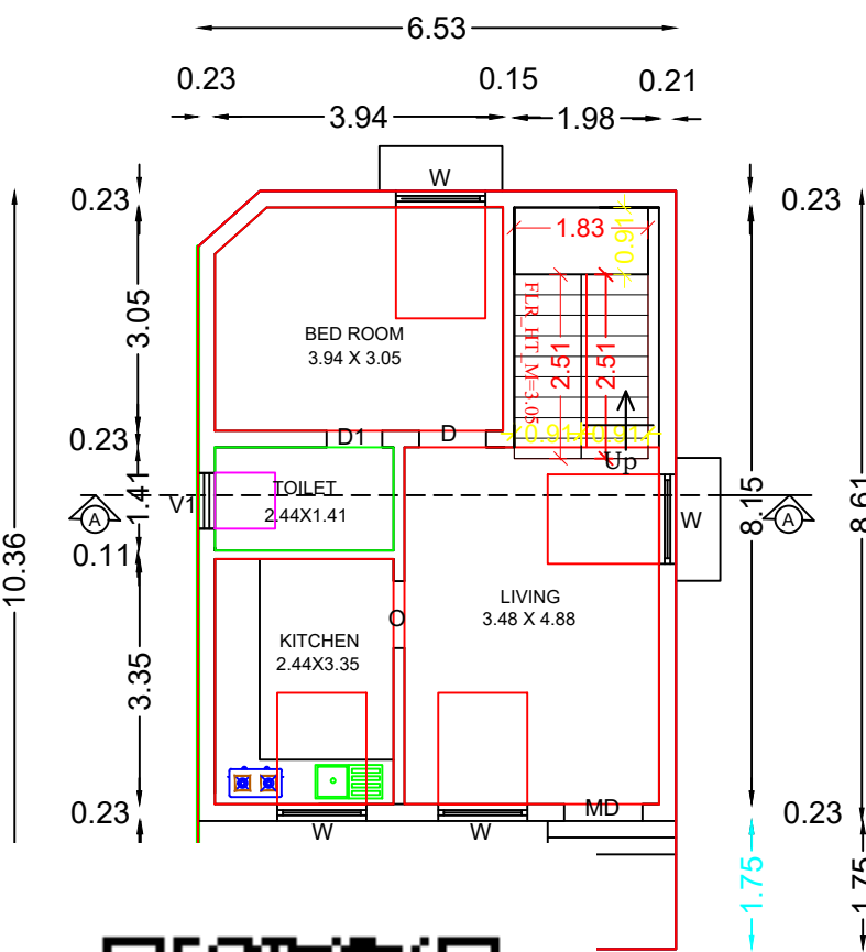
LOOR PLAN
