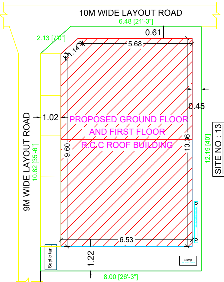
SITE PLAN
