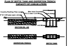
PLAN OF SEPTIC TANK AND DISPERSION TRENCH
