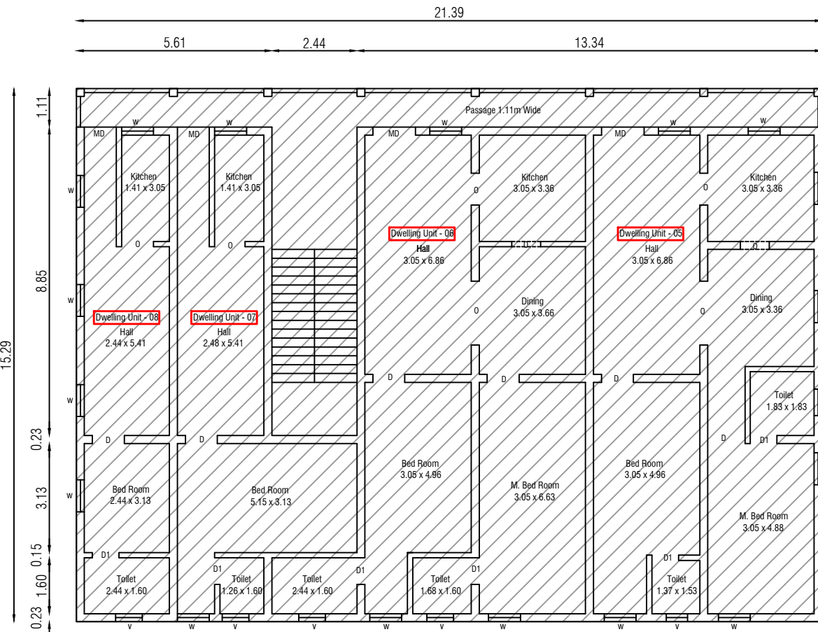
EXISTING & REVISED FIRST FLOOR
