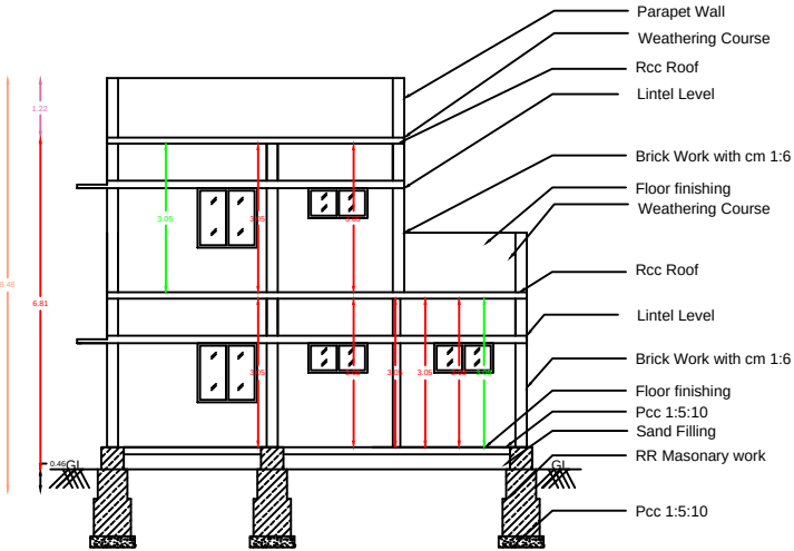
SECTION ON-"AB"
