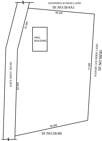
SITE PLAN
