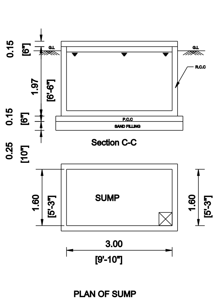
PLAN OF SUMP
