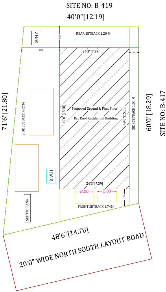
SITE PLAN
