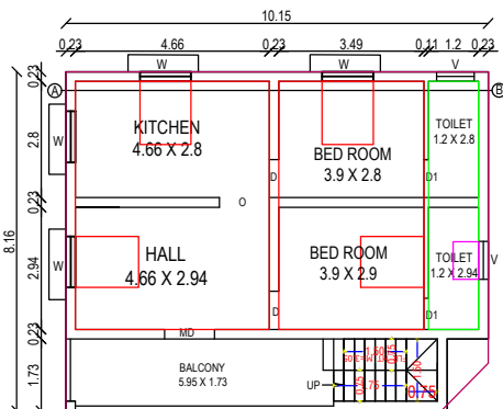
PROPOSED FIRST FLOOR BUILDING
