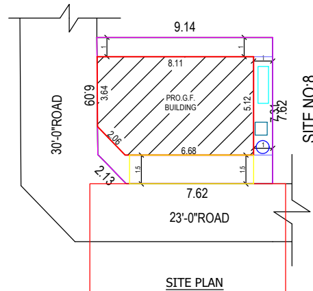
SITE PLAN
