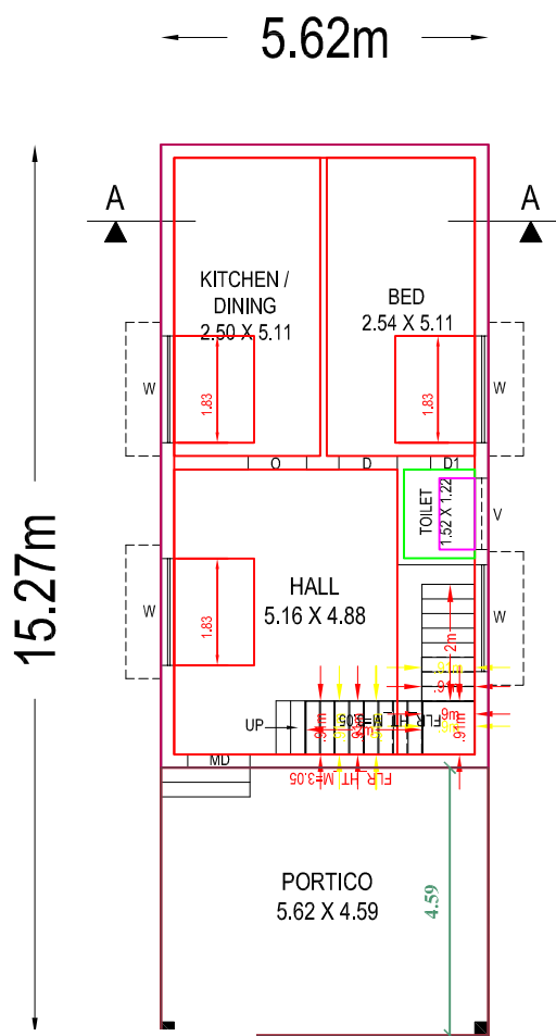
ID FLOOR PLAN
